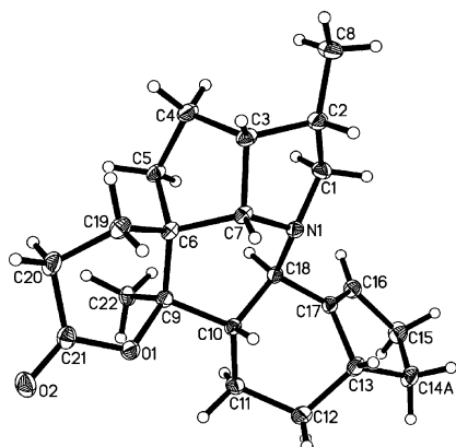
Deoxycalcyciphylline B
